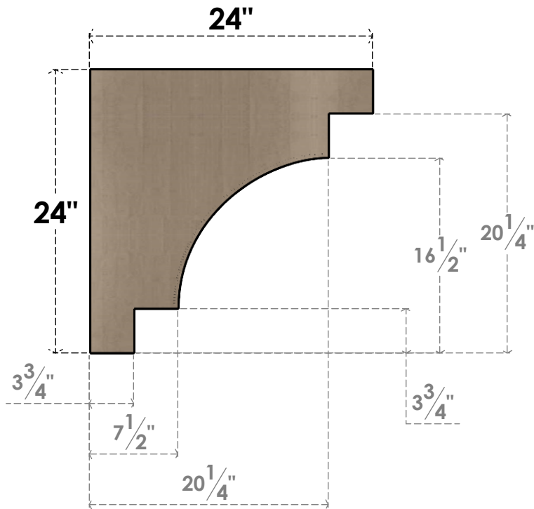
SIDE PROFILE
